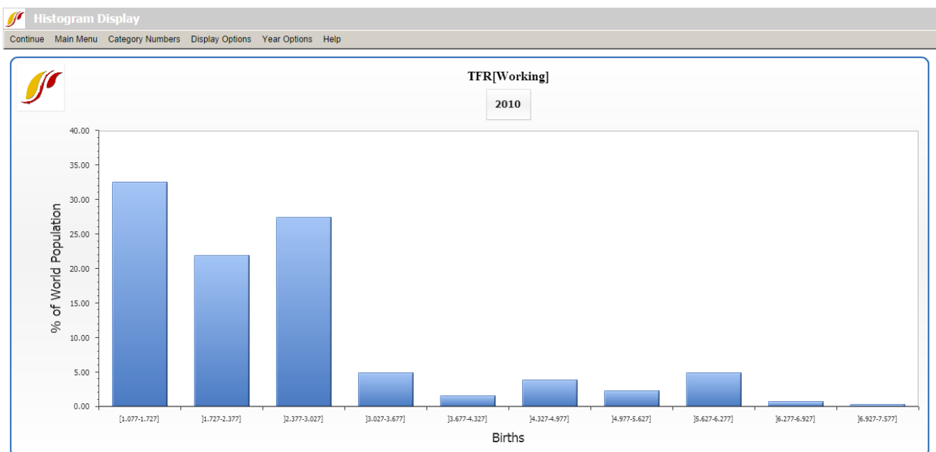
Histogram example
